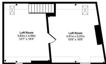
Second Floor Approx 41 sq m / 437 sq ft
